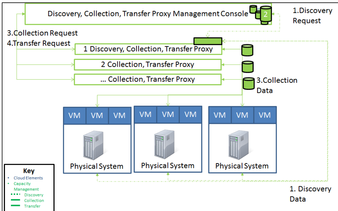
Figure 2: Non-Centrally Managed Cloud Environment Diagram
