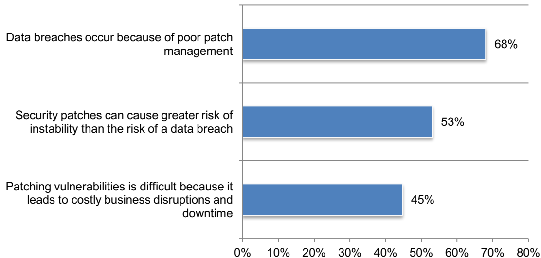
Figure 3. Patching vulnerabilities
